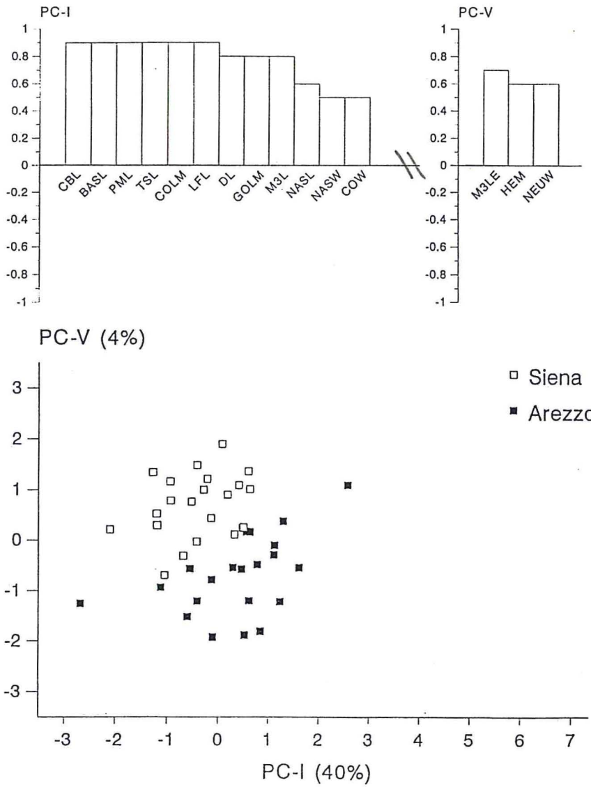
Fig. 4. Principal component analysis of the log.-transformed values of 28 cranial measurements in two roe deer populations of central Italy. The loadings of variables relative to axes I and V are shown in the upper part of the graph (only loadings equal to or greater than 0.5 are shown). The percentage variation explained by each axis is given in parentheses.
